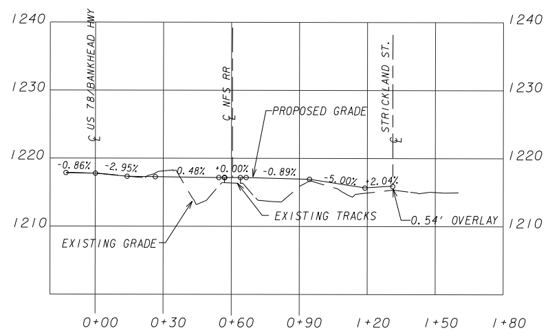
PROFILE McCARLEY STREET RELOCATION HORIZ 1" = 30' VERT 1" = 10'
